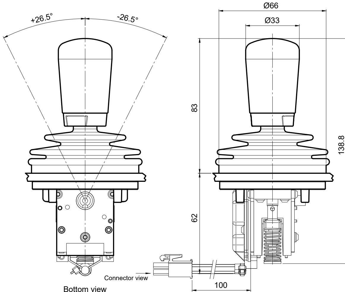
Bottom view
